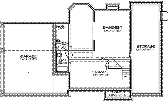
1 FOUNDATION PLAN A-3
