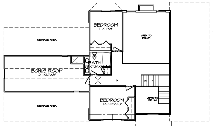
1 SECOND FLOOR PLAN A-5
